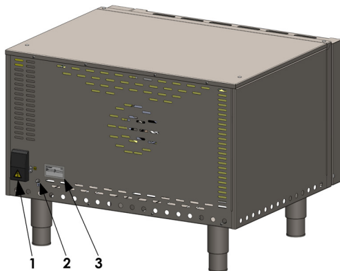
Fig. 4 Connecting the device to an electrical equipotential bonding system
